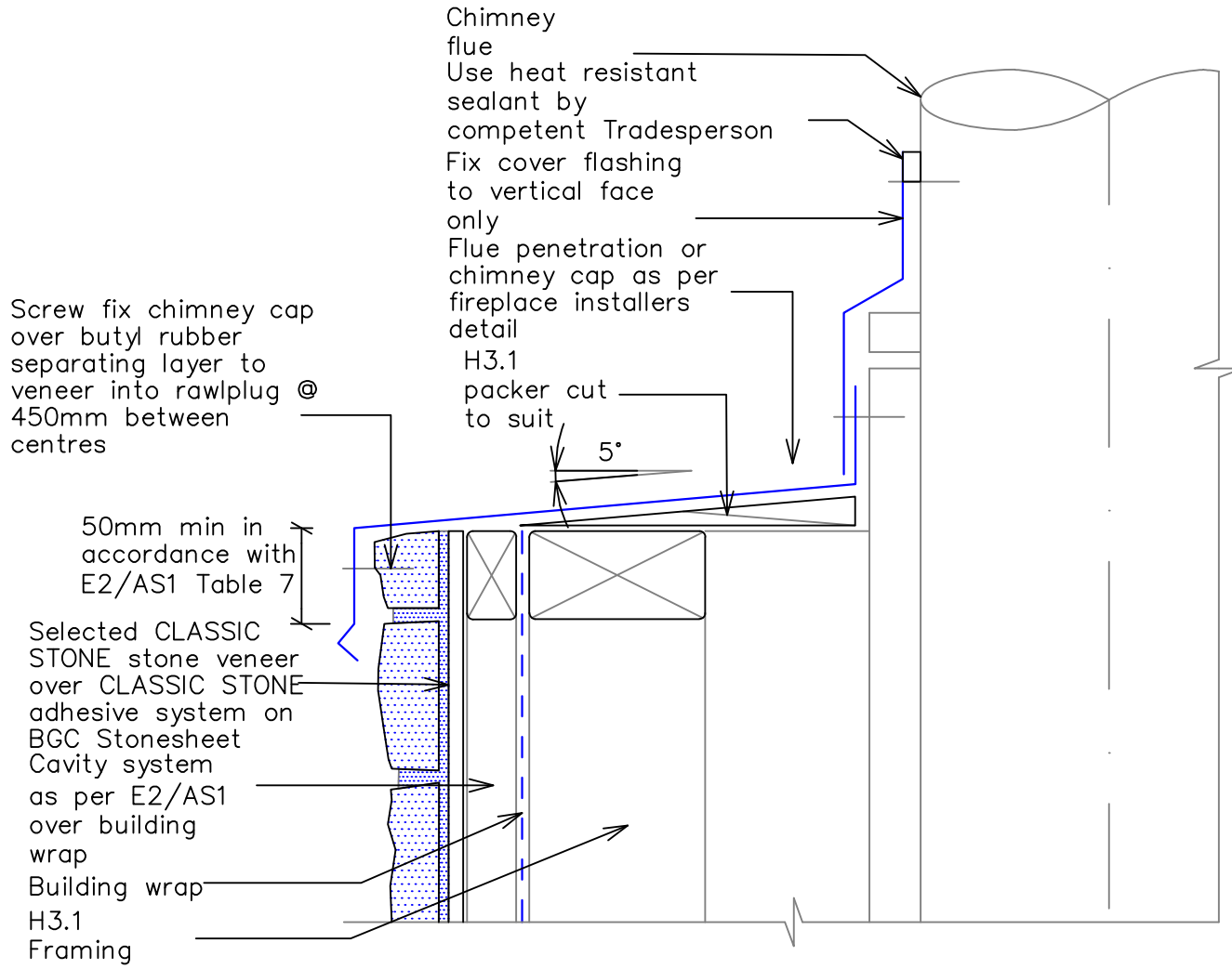
11 – Typical Chimney Cap Detail
