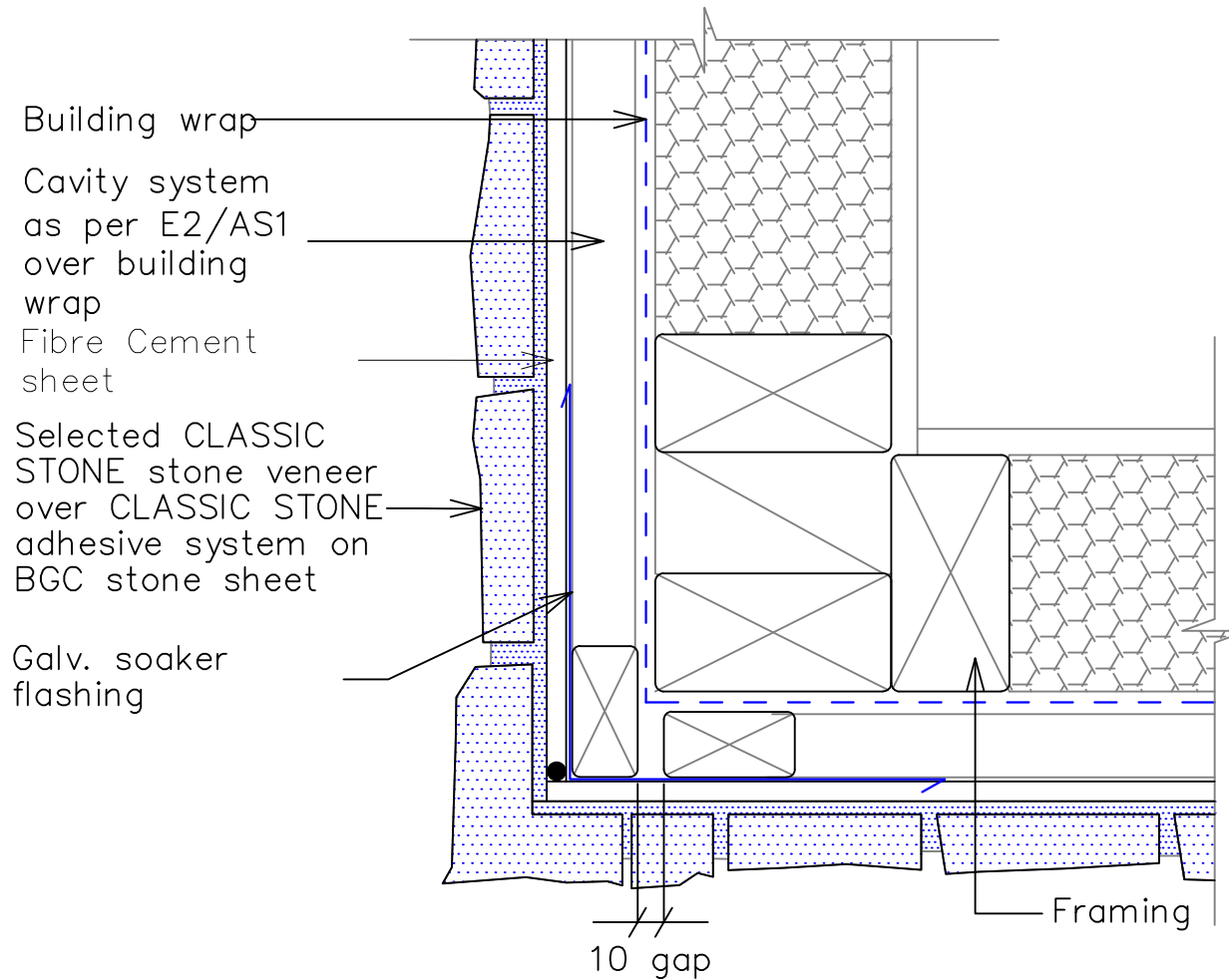
6 – Typical External Corner Detail (plan view)
