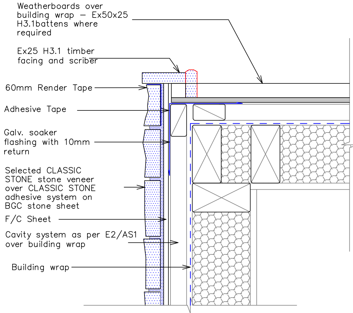
6a – Typical External Corner with Plywood Cladding
