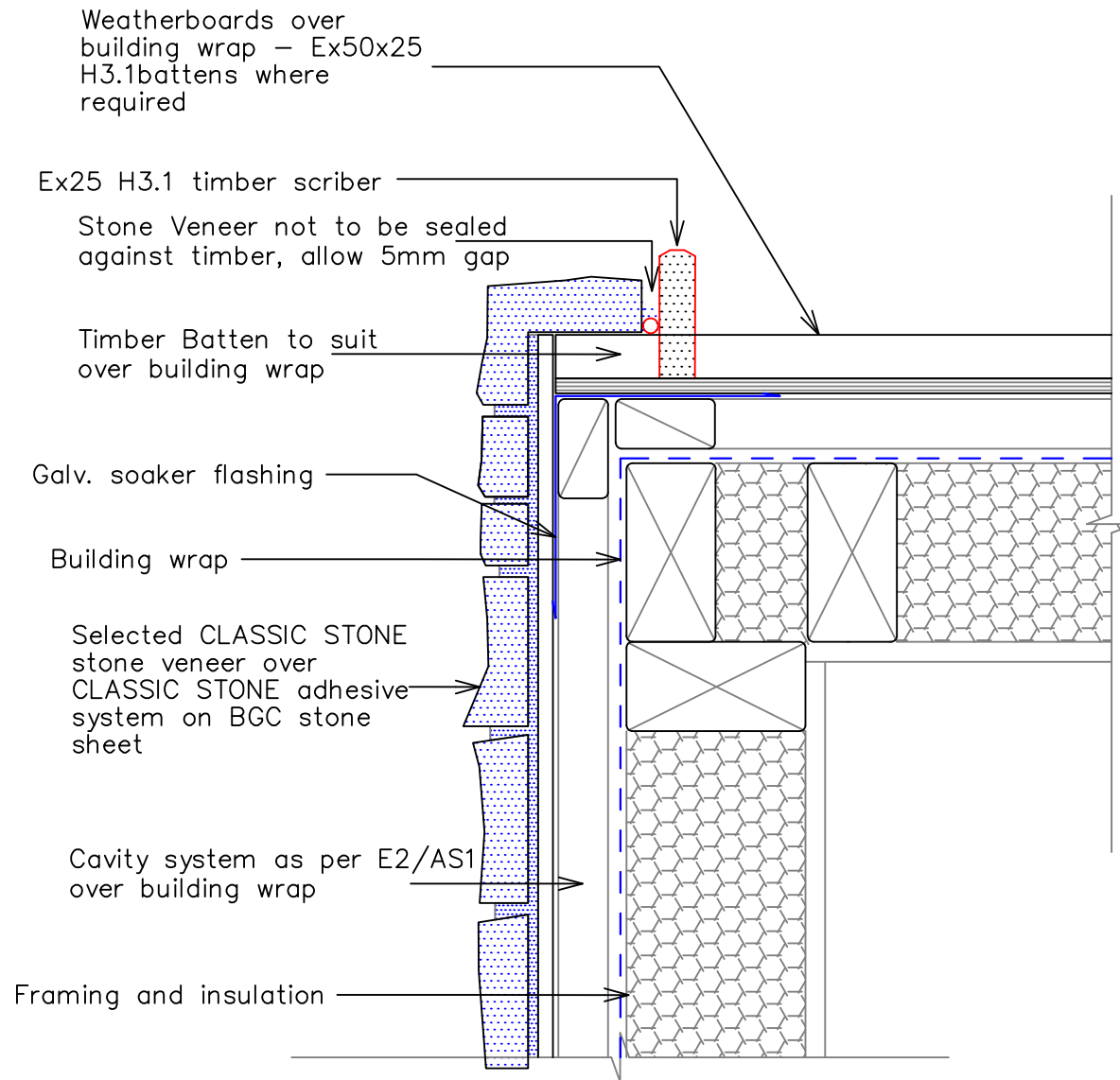
6b – Typical External Corner with Weatherboard
