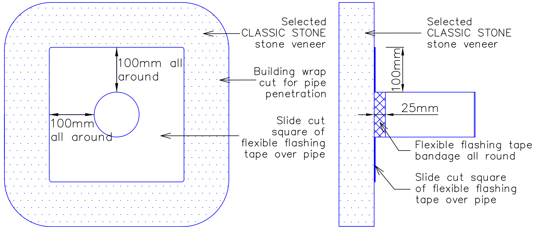
16 – General Pipe Penetration
