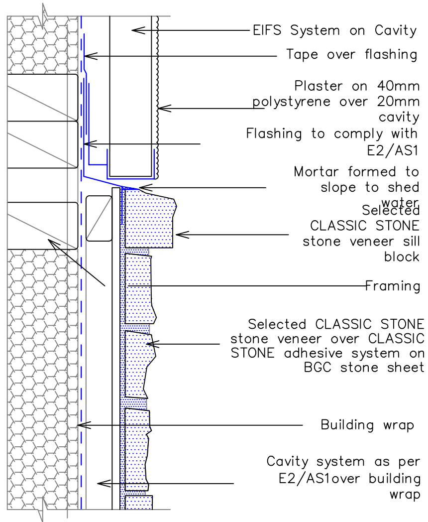
1 – Typical Horizontal Joint with EIFS Cavity System
