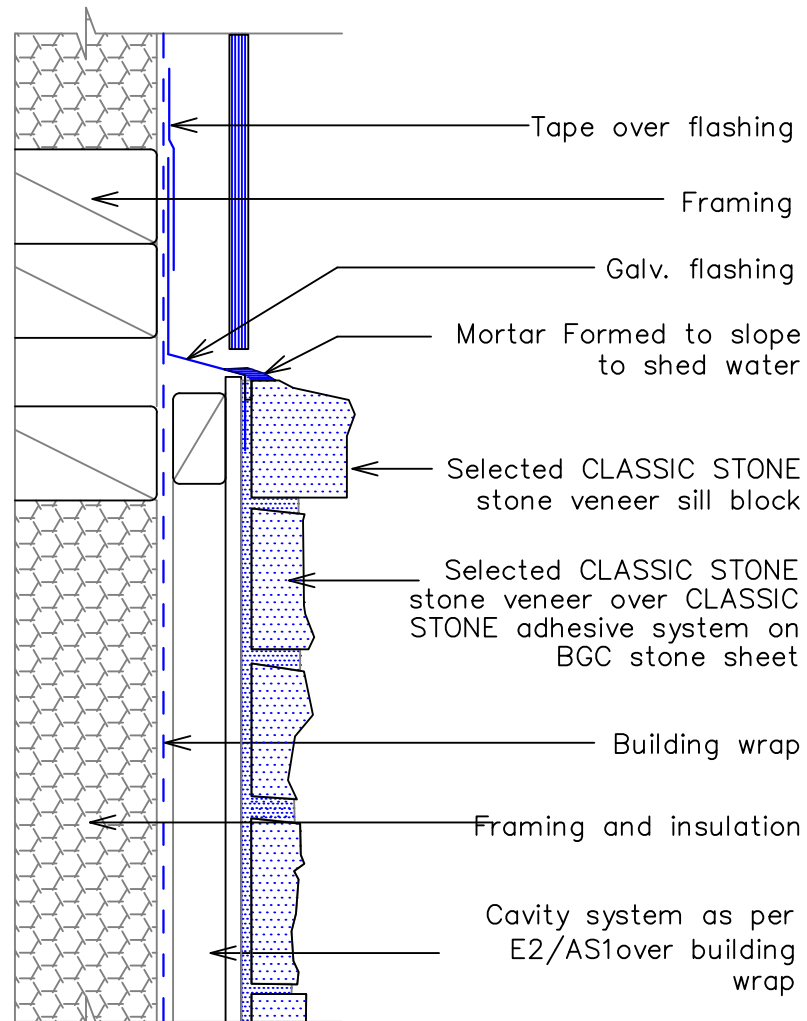
1a - Typical Horizontal Joint with Plywood or fibre cement sheet
