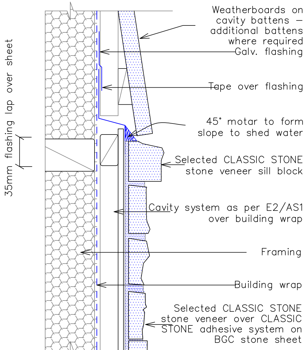
1c – Typical Horizontal Joint with Weatherboard – Cavity
