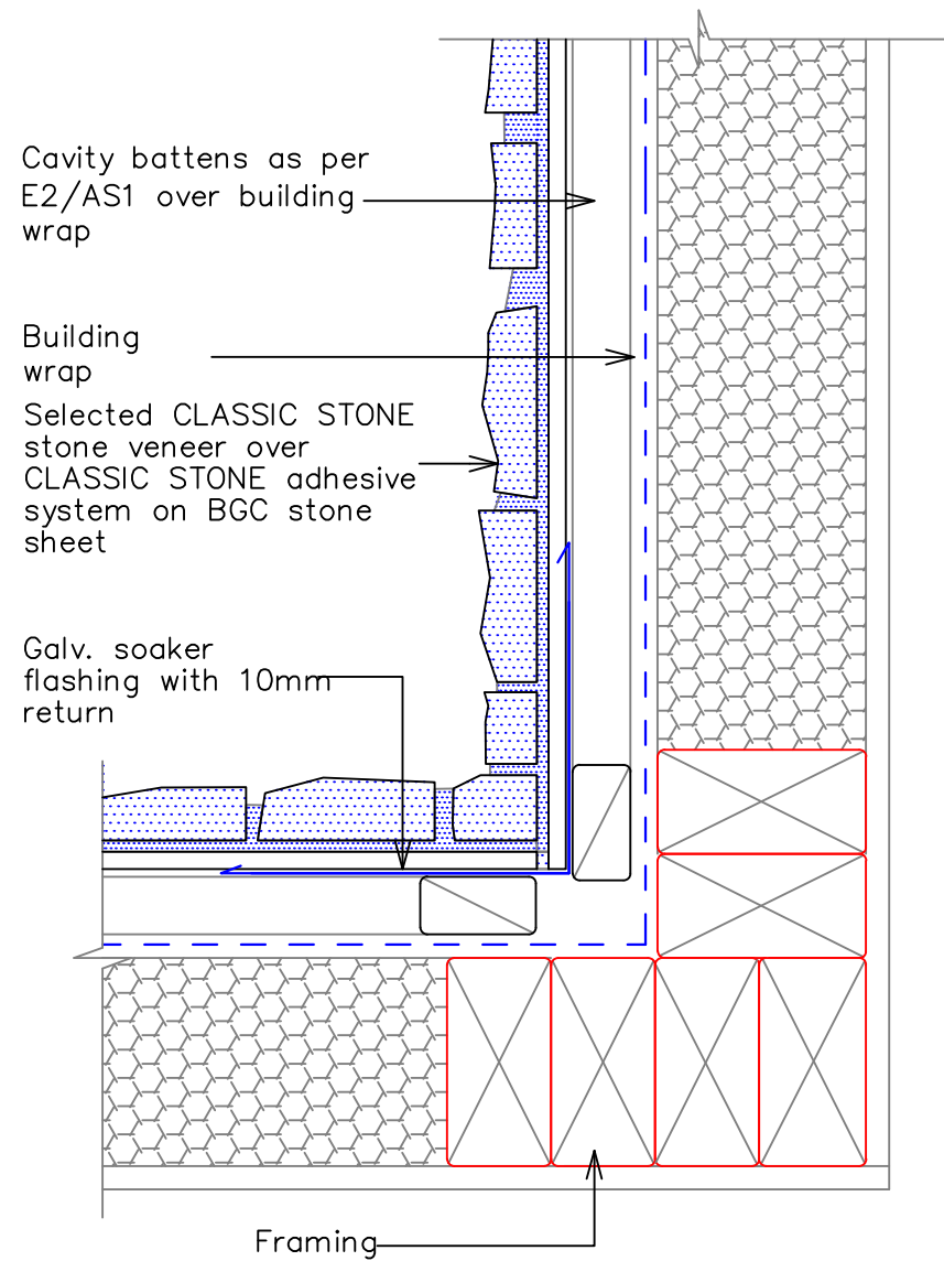
5 – Typical Internal Corner Detail (plan view)
