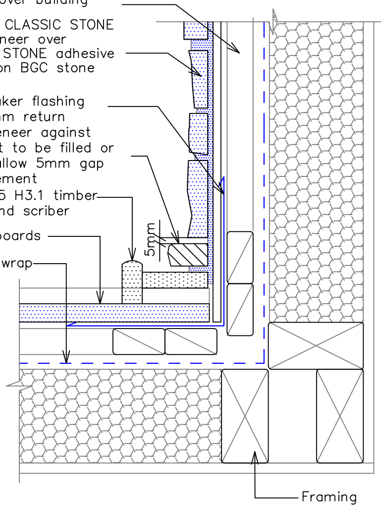
5a – Typical Internal Corner – Weatherboard (plan view)
