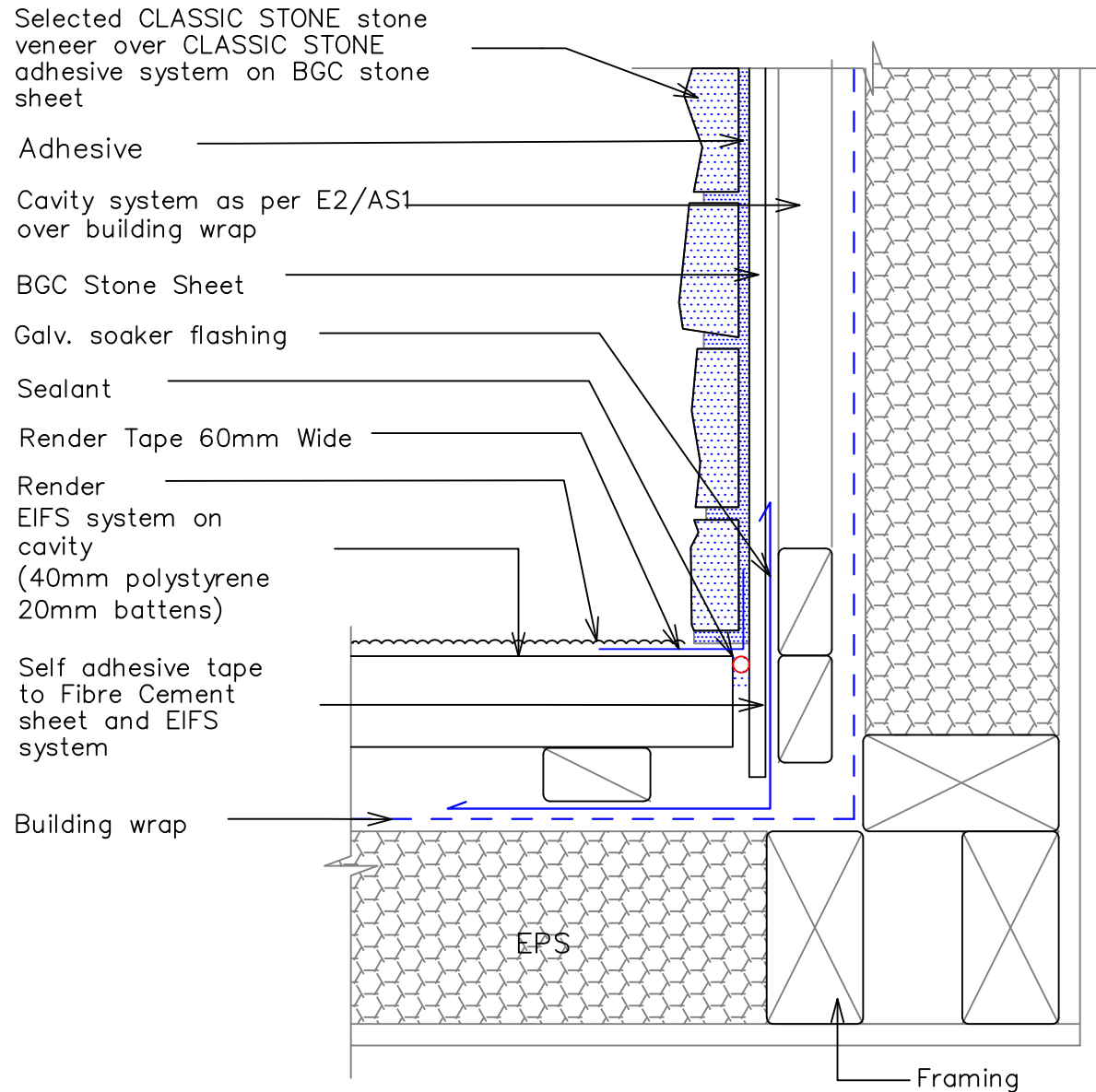
5c – Typical Internal Corner with EIFS Cavity System (plan view)
