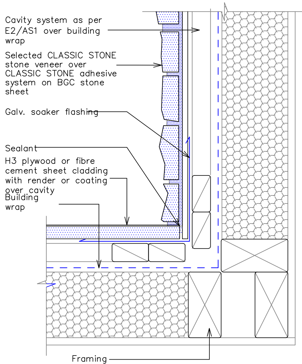
5b – Typical Internal Corner – Plywood or fibre cement with render or coating Sheet
