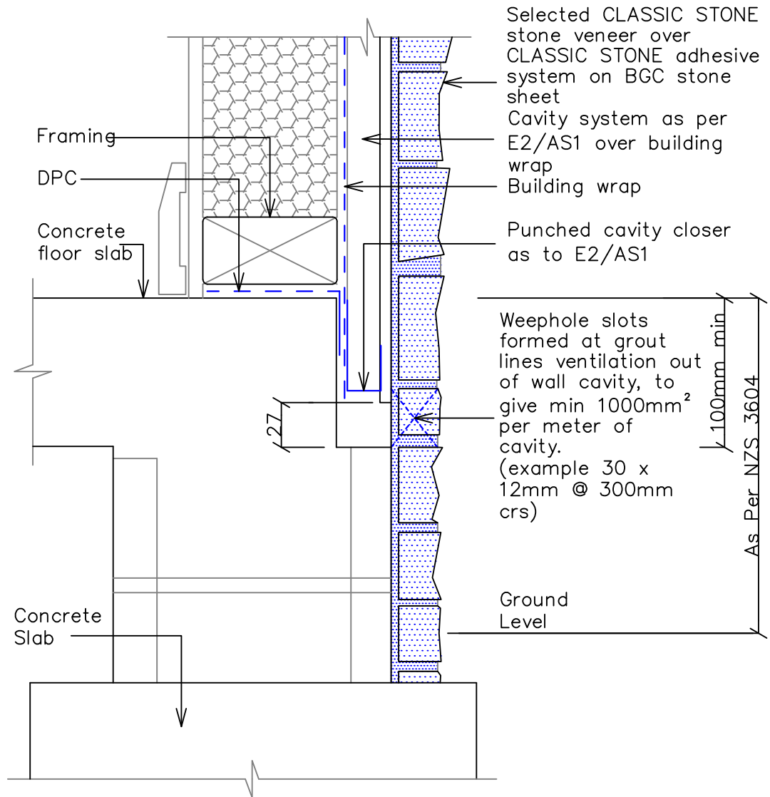
9a – Typical Rebated Slab Edge Detail
