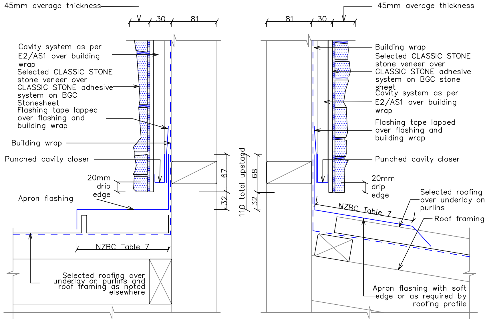
10 – Typical Roof Abutment Detail
