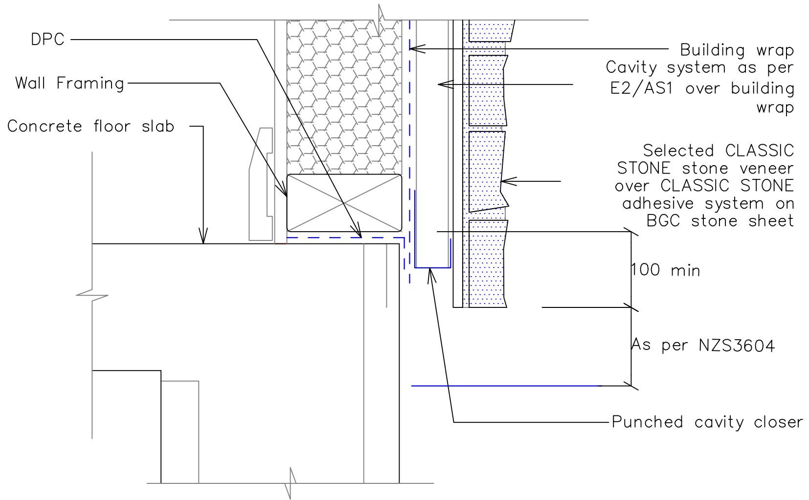
9 – Typical Slab Edge Detail
