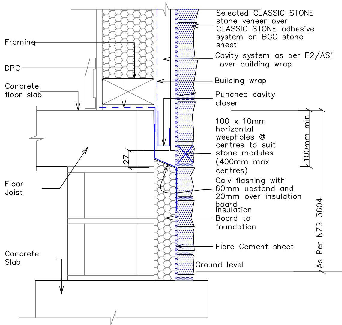
9c – Typical Slab Edge Detail (with weepholes)
