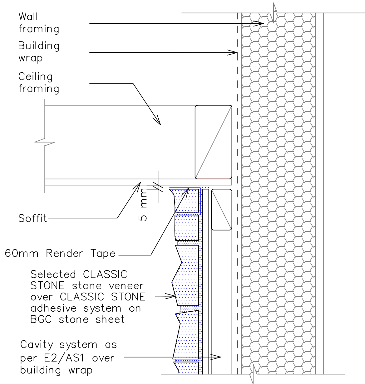
8 – Typical Soffit Detail
