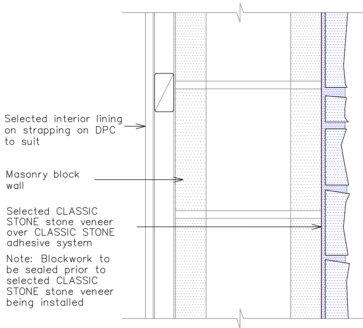
12 – Typical Stone Veneer over Block Wall
