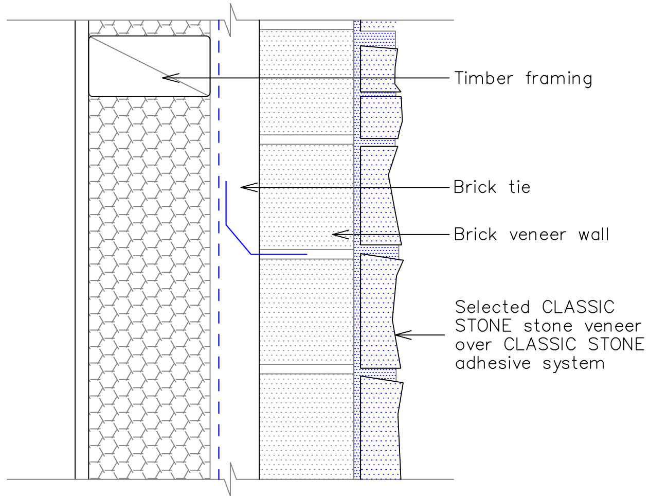
13 – Typical Stone Veneer over Brickwork
