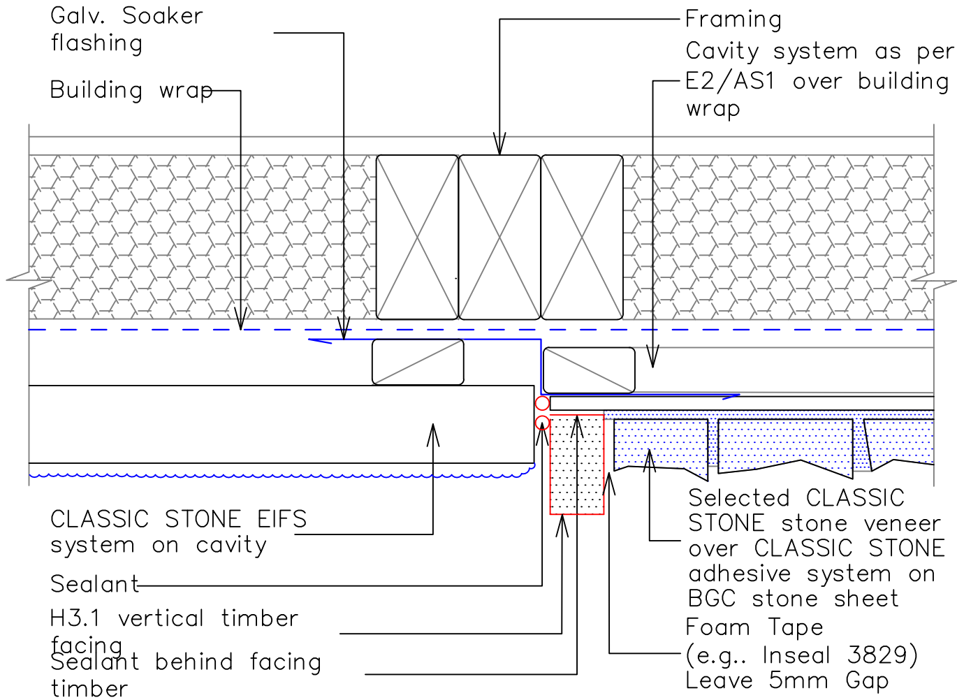
7c – Typical Vertical Joint – Stone Veneer to EIFS Cavity System
