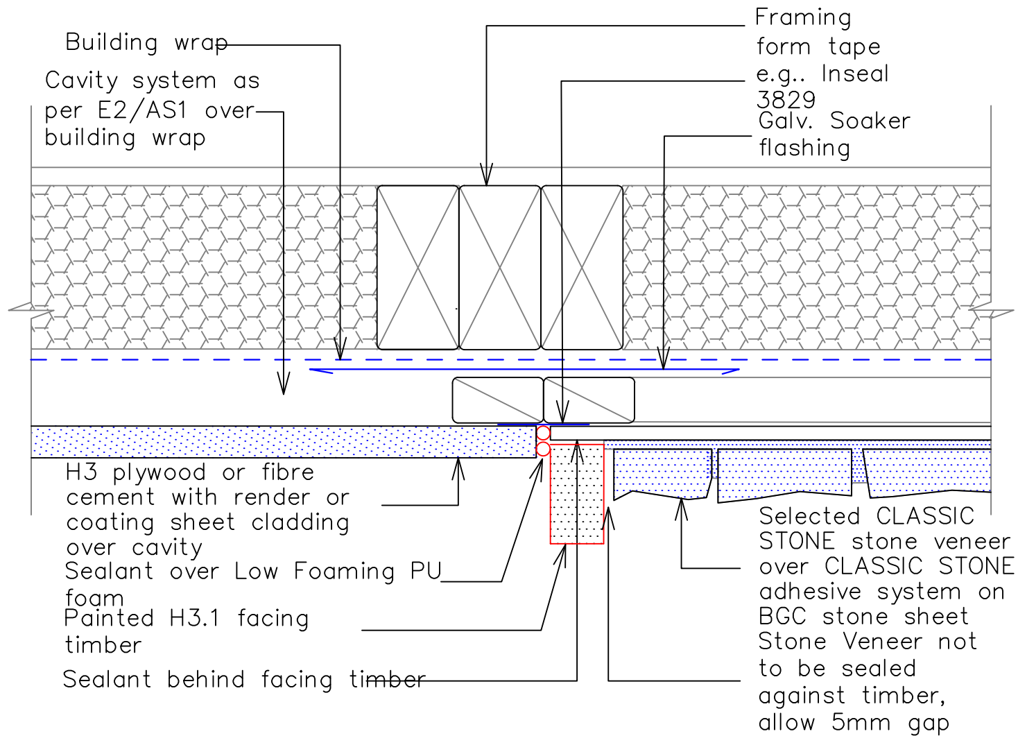
7b – Typical Vertical Joint – Stone Veneer to Plywood or fibre cement sheet with render or coating
