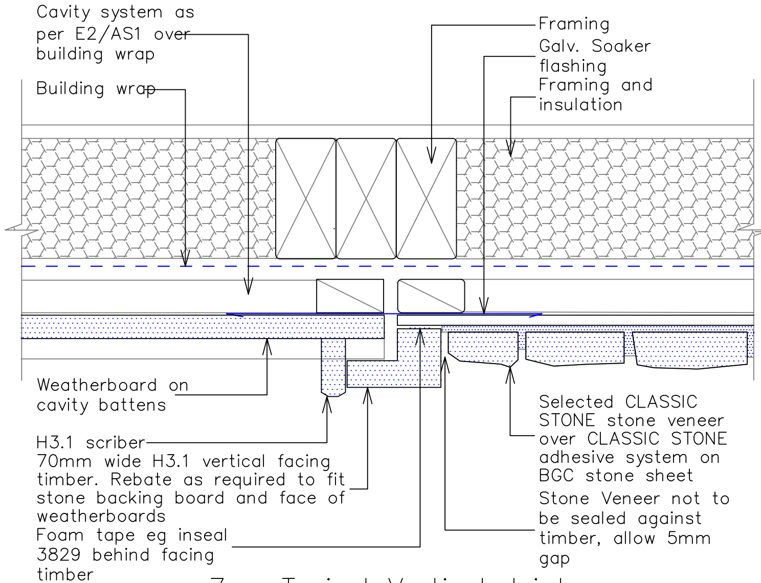
7 – Typical Vertical Joint – Stone Veneer to Weatherboard – Cavity (plan view)
