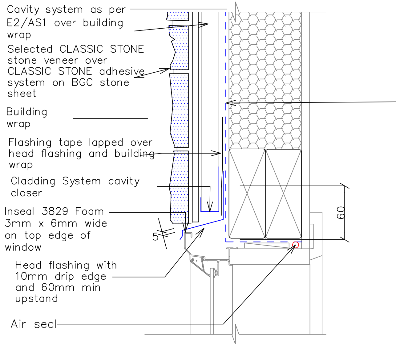
3 – Typical Window Head Detail
