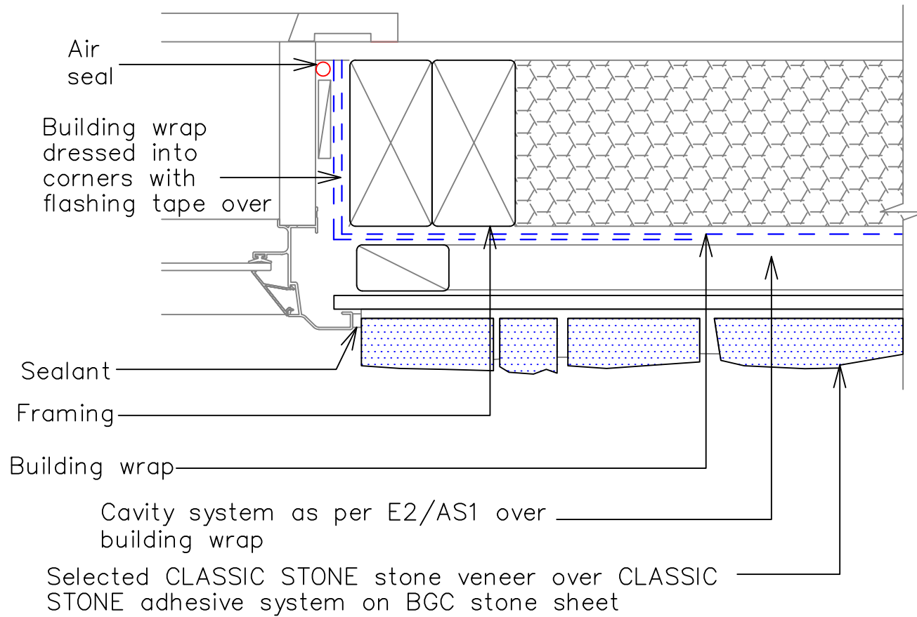
4 – Typical Window Jamb Detail
