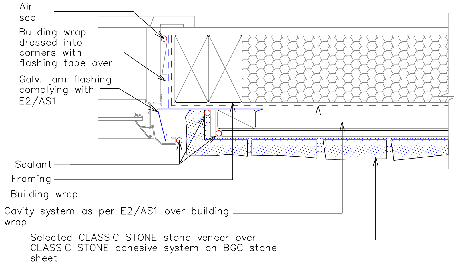
4a – Typical Window Jamb Detail – Recessed (plan view)
