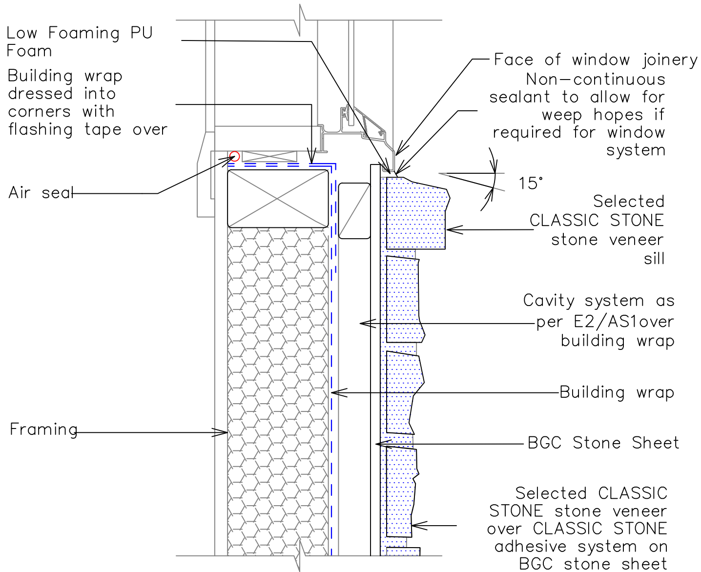
2 – Typical Window Sill
