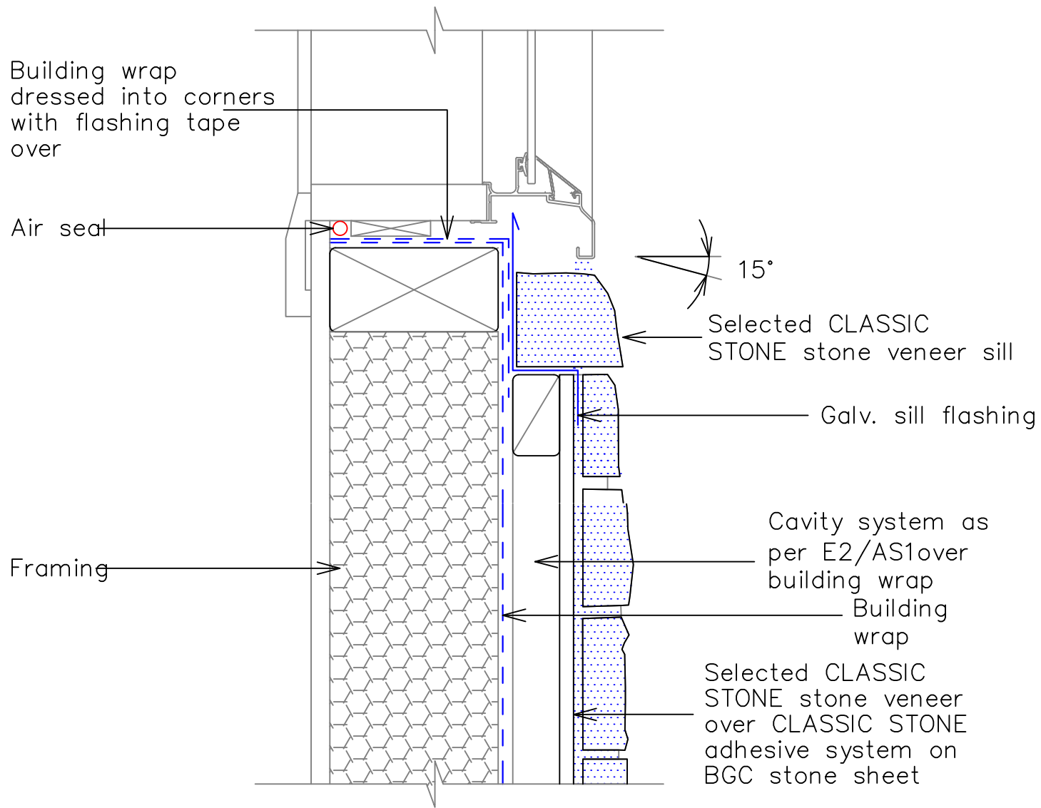
2a – Typical Window Sill – Recessed
