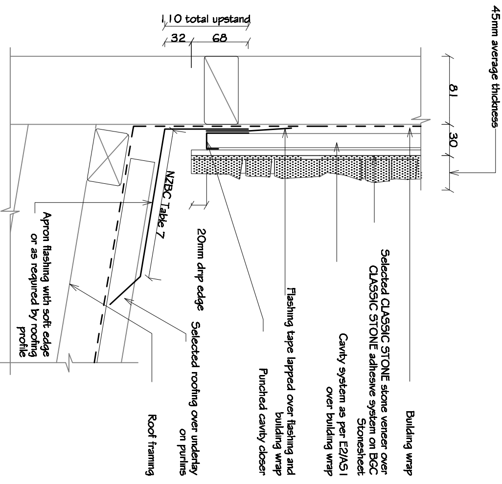
10 - Typical Roof Abutment Detail
